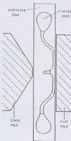
Figure 2. The development of 2 D front boundary from the centre in inhomogeneous magnetic field.
